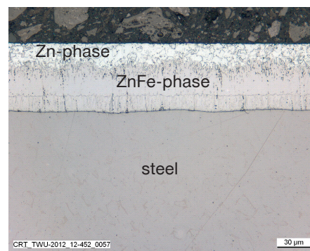
Fig. 30: Micrograph of hot-dip galvanized steel.
