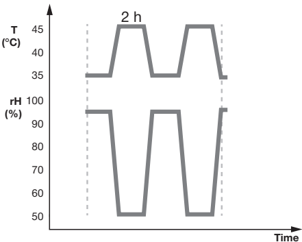
Fig. 16: Daily temperature and humidity cycle of the ISO 16701 cyclic corrosion test: twice a week, a 1 % NaCl solution is sprayed onto the samples for 3 × 15 minutes.
